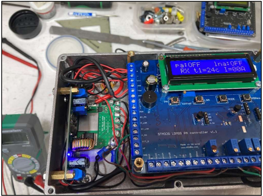
Figure 6 Control Board Installation
