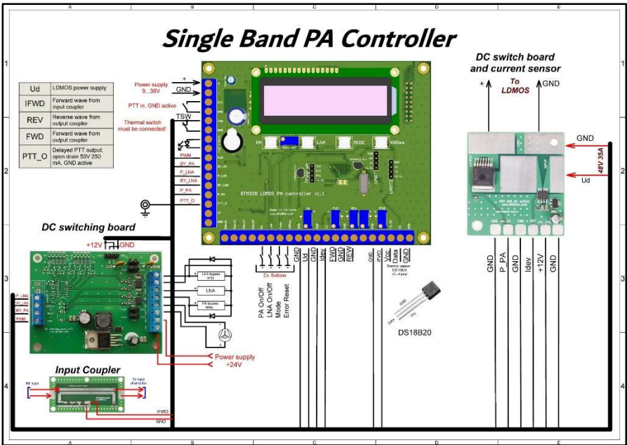
Figure 5 Control Board
